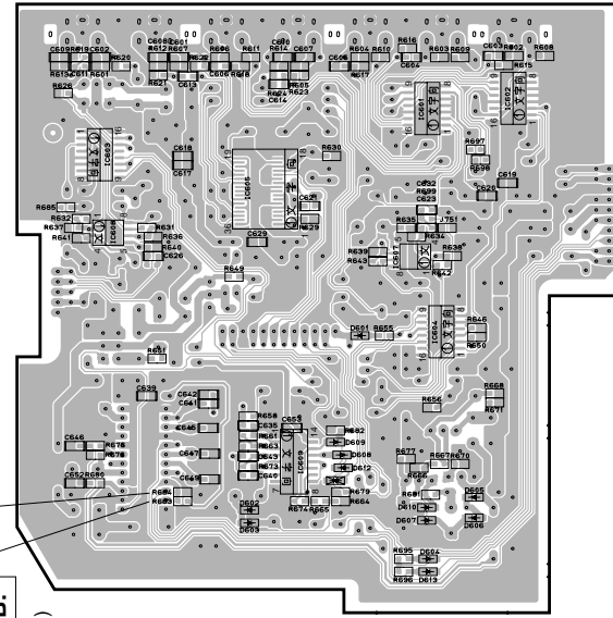
FUNCTION (3) P.C.B. (Surface Mount Device)
