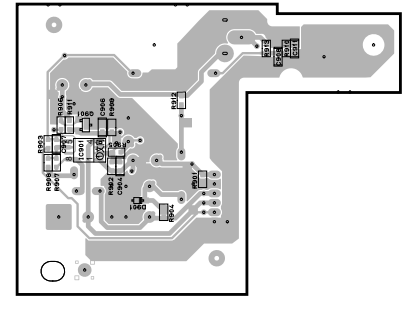
OPERATION (5) P.C.B.
