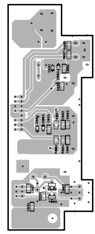
OPERATION (4) P.C.B.
