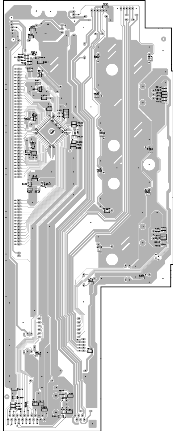
OPERATION (1) P.C.B. (Surface Mount Device)
